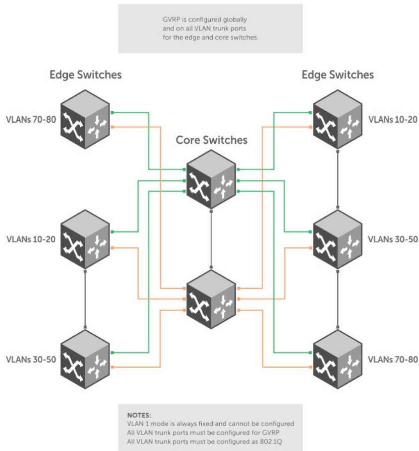
Figure 36. Global GVRP Configuration Example
